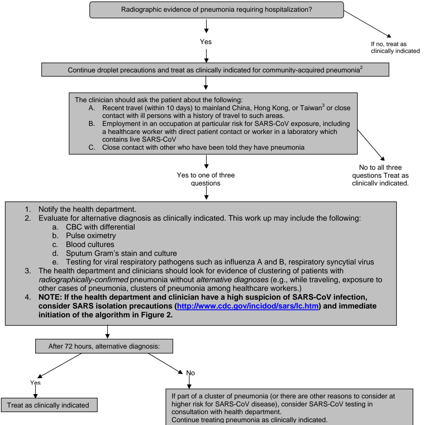
Figure 1. Algorithm for evaluation and management of patients requiring hospitalization for radiographically confirmed pneumonia, in the absence of person-to-person transmission of SARS-CoV in the world
